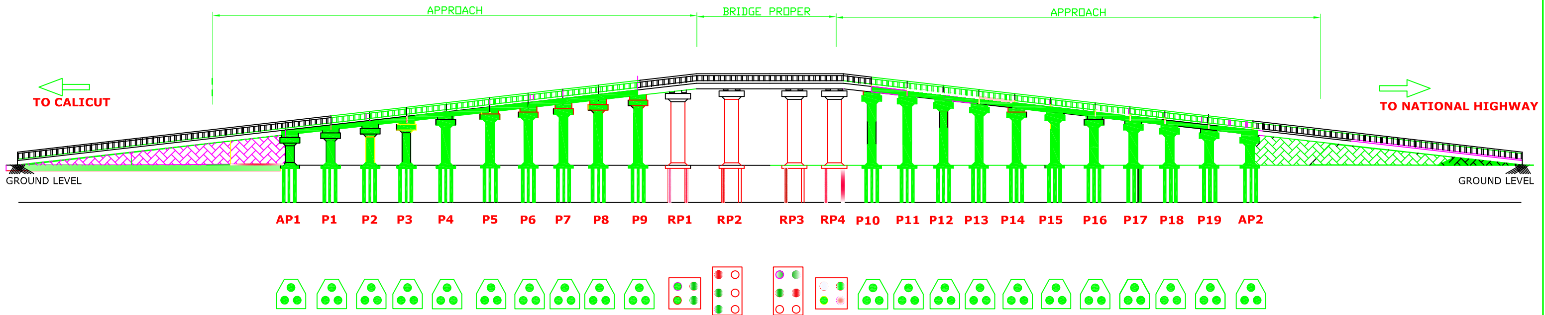
PILE FOUNDATION
